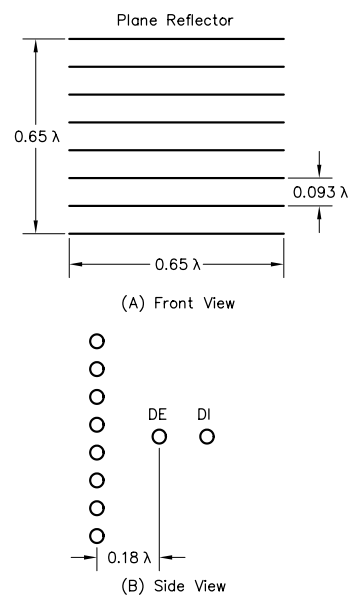
Fig 30 —Front and side views of a plane-reflector antenna.
