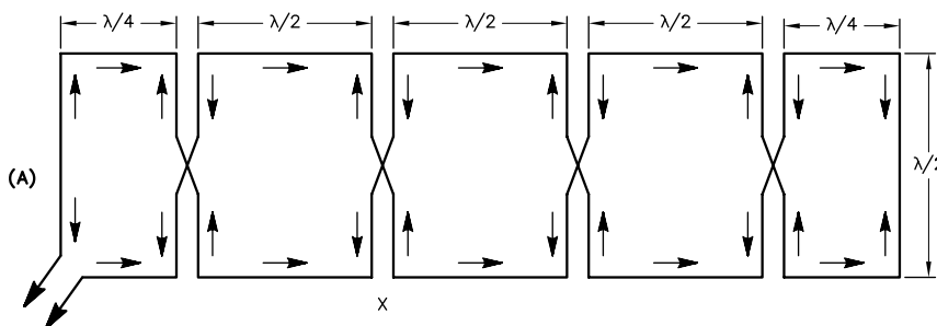
Fig 46 —Typical Sterba array, a 10-element version.
