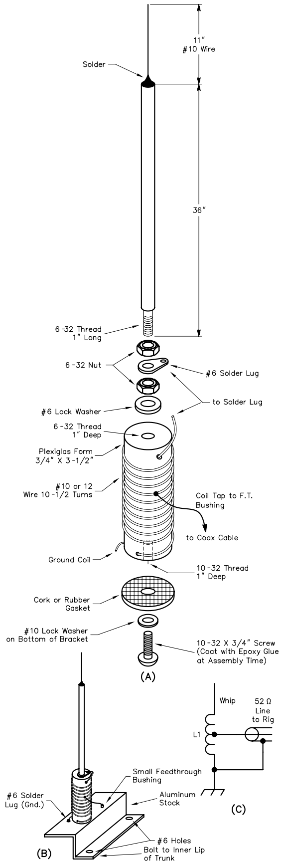
Fig 50 —Structural details for the 2-meter \frac{5}{8}\lambda antenna are provided at A. The mounting bracket is shown at B and the equivalent circuit is given at C.
