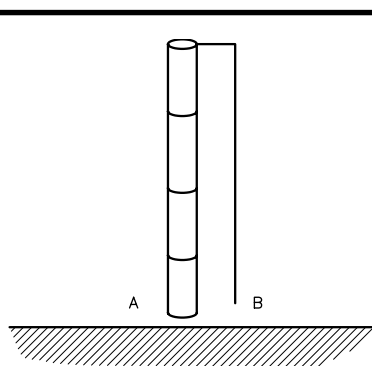
Fig 40—Vertical ground-plane antenna with a 10-foot pipe and #12 wire as the linear-loaded element. Resonant frequency and radiation resistance depend on which side (A or B) is fed. The other side (B or A) is not grounded. See text for details.
