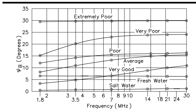
Fig 8 —Pseudo-Brewster angle ( \Psi ) for various qualities of earth over the 1.8 to 30-MHz frequency range. Note that the frequency scale is logarithmic. The constants used for each curve are given in Table 2.
