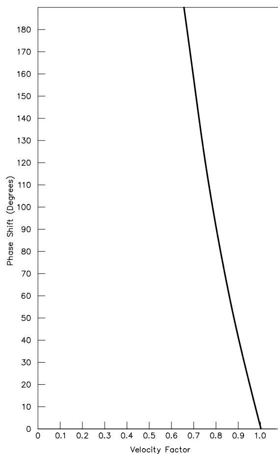
Fig 33—This curve shows phase shift (per wavelength) as a function of velocity factor on a Beverage antenna. Once the phase shift for the antenna goes beyond 90^\circ , the gain drops off from its peak value, and any increase in antenna length will decrease gain.
