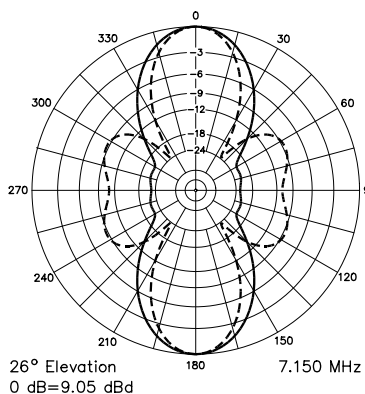
Fig 6 —Azimuth pattern for N6LF Double Extended Zepp (solid line), compared to classic Double Extended Zepp (dashed line). The main lobe for the modified antenna is slightly broader than that of the classic model, and the sidelobes are suppressed better.
