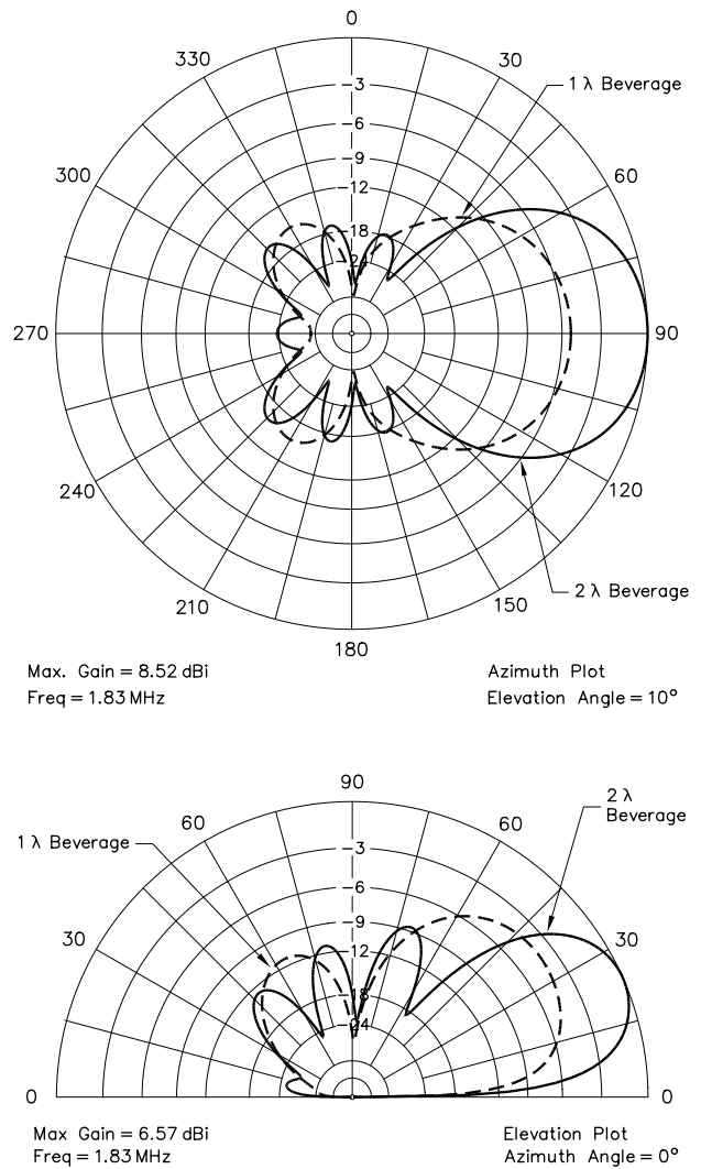
Fig 35 —At top, azimuthal patterns of a 2- \lambda (solid line) and a 1- \lambda (dashed line) Beverage antenna, terminated with 550- \Omega resistor at 1.83 MHz, at an elevation angle of 10°. The rearward pattern around 180° is more than 20 dB down from the front lobe for each antenna. Above, the elevation-plane patterns. Note the rejection of very high-angle signals near 90°.
