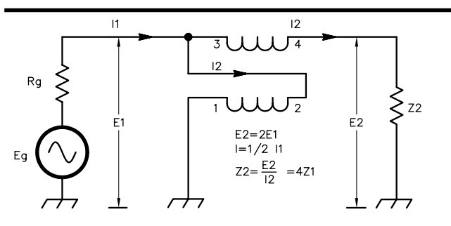
Fig 21—Broadband bifilar transformer with a 4:1 impedance ratio. The upper winding can be tapped at appropriate points to obtain other ratios such as 1.5:1, 2:1 and 3:1.
