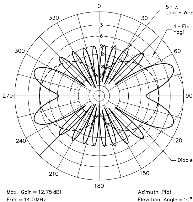
Fig 6—At left, the azimuth responses for a 5-λ long-wire (350 feet long at 14 MHz—solid line) to the same 4-element Yagi (dotted line) and dipole (dashed line) as in Fig 5. Above, the elevation-plane responses for the long-wire (solid line) and the dipole (dashed line) by themselves. Note that the elevation angle giving peak gain for each antenna is just about the same. The long-wire achieves gain by compressing mainly the azimuthal response, squeezing the gain into narrow lobes; not so much by squeezing the elevation pattern for gain.
