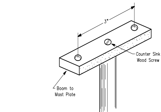
Fig 54—Boom-to-mast plate for the 144-MHz quad. The screw hole in the center of the plate should be countersunk so the wood screw attaching it to the mast does not interfere with the fit of the boom.
