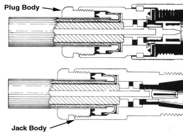
Fig 29—Type N connectors are required for high-power operation at VHF and UHF. (Courtesy of Amphenol Electronic Components, RF Division, Bunker Ramo Corp.)
