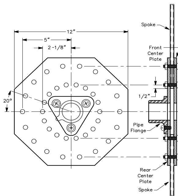
Fig 29—Center plate details. Two center plates are bolted together to hold the spokes in place.
