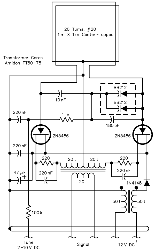
Fig 66—Remote active preamplifier for directional loop receiving antenna.
