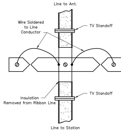
Fig 20—The lightning arrester of Fig 19 may be used with 300- \Omega ribbon line in the manner shown here. The TV standoffs support the line an inch or so away from the grounded center member of the arrester.
