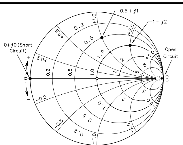
Fig 3 —The complete coordinate system of the Smith Chart. For simplicity, only a few divisions are shown for the resistance and reactance values. Various types of Smith Chart forms are available from ARRL HQ. At the time of this writing, five 8½ × 11 inch Smith Chart forms are available for $2.
