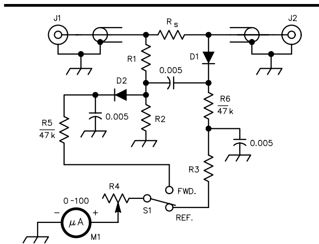
Fig 5—Resistance bridge for SWR measurement. Capacitors are disc ceramic. Resistors are 1/2-watt composition except as noted below.
