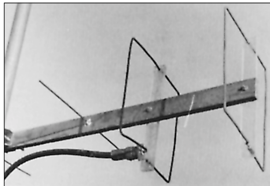
Fig 57—A close-up view of the feed method used on a 432-MHz Quagi. This arrangement produces a low SWR and gain in excess of 13 dBi with a 4-foot 10-inch boom! The same basic arrangement is used on lower frequencies, but wood may be substituted for the Plexiglas spreaders. The boom is 1 / 2 -inch exterior plywood.
