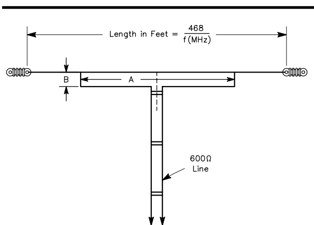
Fig 9—The T matching system, applied to a 1/2\text{-}\lambda antenna and 600- \Omega line.
