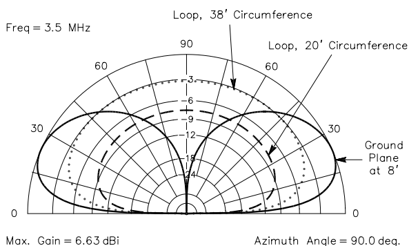
Fig 18—Elevation-plane response of three antennas at 3.5 MHz—a 20-foot circumference octagonal copper loop, a 38-foot circumference copper loop and a full-sized λ/4 ground plane with two elevated radials. The bottom of each antenna is mounted 8 feet above ground for safety. The 38-foot circumference loop (which has a “wingspan” of 11.5 feet) is fairly competitive with the much large ground-plane, being down only about 4 dB at low elevation angles. The 20-foot circumference loop is much more lossy, but with its top only about 14 feet off the ground is very much of a “stealth” antenna.
