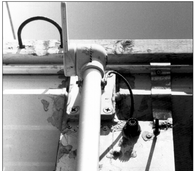
Fig 12 —Photo of aluminum base plate, showing details of mounting to the camper. The four banana-plug jacks on the bottom are for extra radials, if desired.
