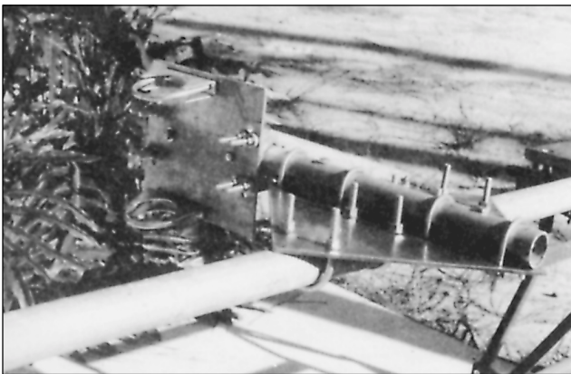
Fig 38—Close-up of the PVRC mount. The long pipe (horizontal in this photo) is the rotating mast. The U bolts in the vertical plate at the left are ready to accept the antenna boom. The heads of two locking pins (bolts) are visible at the midline of the boom plate. The other two pins help secure the horizontal pipe to the large steel mast plate. (The head of the bolt nearest the camera blends in with the right hand leg of the U bolt behind it.)
