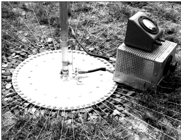
Fig 45—Base of the vertical antenna showing the 60 radial wires. The aluminum disc is 15 inches in diameter and \frac{1}{4} inches thick. Sixty tapped holes for \frac{1}{4} -20 aluminum hex-head bolts form the outer ring and 20 form the inner ring. The inner bolts were used for performance comparisons with more than 60 radials. The insulator is polystyrene material (phenolic or Plexiglas suitable) with a 1-inch diameter. Also shown is the impedance bridge used for measuring input resistance.
