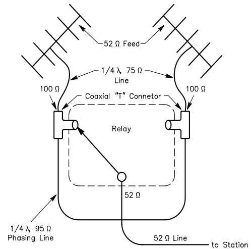
Fig 21—Electrical diagram of the switchable polarization antenna system, complete with cable specifications. When calculating the lengths of individual cables, be sure to include the proper velocity factor of the cable used.
