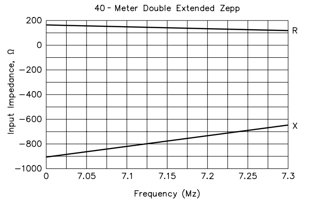
Fig 45 —Resistive and reactive feed-point impedance of a 40-meter extended double Zepp in free space.
