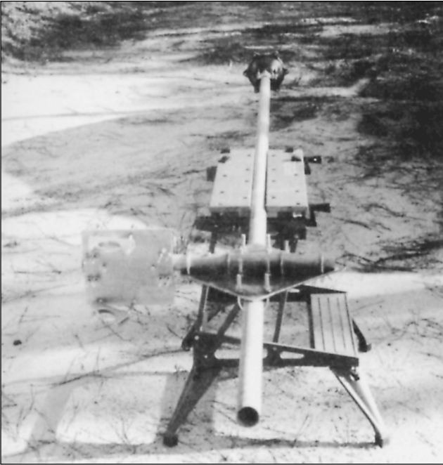
Fig 37—The PVRC mount, boom plate, mast and rotator ready to go. The mast and rotator are installed on the tower first.
