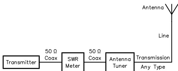
Fig 1—Essentials of a coupling system between transmitter and transmission line.
