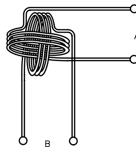
Fig 10—An early type of goniometer that is still used today in some RDF applications. This device is a special type of RF transformer that permits a movable coil in the center (not shown here) to be rotated and determine directions even though the elements are stationary.
