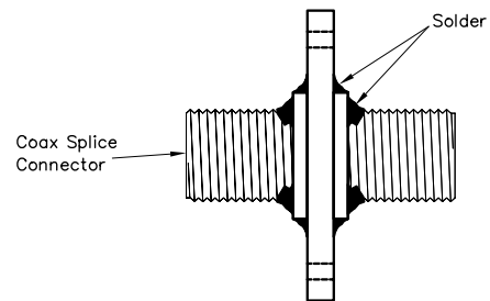
Fig 18—Feedthrough connector for coax line. An Amphenol 83-1J (PL-258) connector, the type used to splice sections of coax line together, is soldered into a hole cut in a brass mounting flange. An Amphenol bulkhead adapter 83-1F may be used instead.
