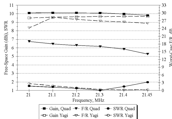
Fig 4—Comparison of gain, F/R and SWR over the 21.0 to 21.45-MHz range for an optimized 5-element quad and optimized 5-element Yagi, both on 26-foot booms. The quad enjoys a gain advantage of about 0.5 dB over most of the band. Its rearward pattern is not as good as the Yagi, which remains higher than 24 dB across the whole range, compared to the quad, which remains in the 16-dB average range.
