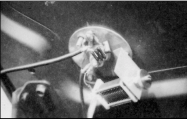
Fig 30 —Details of the matching network located at the base of the antenna inside the vehicle. The mica capacitors are visible at the center. The coaxial stub used to switch them in and out of the circuit comes in from the left, and the feed line exits toward the bottom of the photo.
