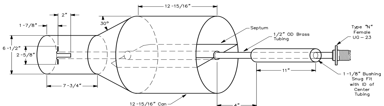
Fig 31 —Backfire type 1296-MHz feed horn, linear polarization only. The small can is a Quaker State oil container; the large can is a 50-pound shortening container (obtained from a restaurant, Gold Crisp brand). Brass tubing, \frac{1}{2} -inch OD, extends from UG-23 connector to dipole. Center conductor and dielectric are obtained from \frac{3}{8} -inch Alumafom coaxial cable. The dipole is made from \frac{3}{32} -inch copper rod. The septum and 30° section are made from galvanized sheet metal. Styrofoam is used to hold the septum in position. The primary gain is 12.2 dBi.
