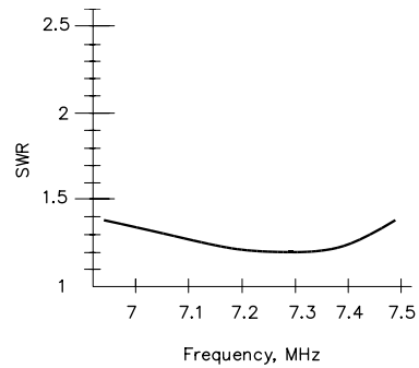
Fig 8— Measured SWR curve across 40-meter band for N6LF DEZepp.
