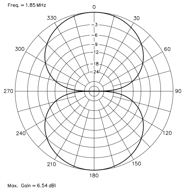
Fig 75 —Free-space E-plane pattern for the antenna shown in Fig 74 , with 1/8\lambda spacing. The elements are parallel to the 90^\circ - 270^\circ line in this diagram. Less than a 1^\circ change in half-power beamwidth results when the spacing is changed from 1/8 to 1/4\lambda .
