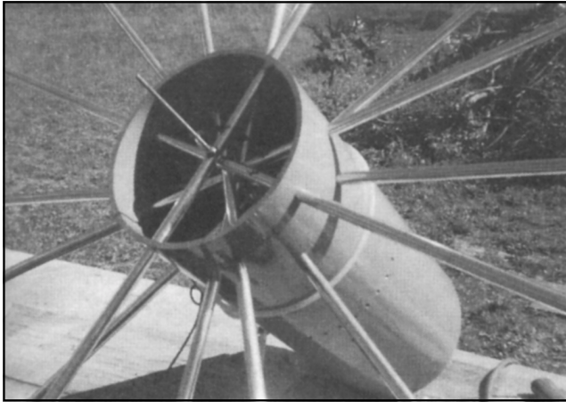
Fig 46—Photo showing details of the hub assembly for the large dish, including the threaded brass rod that connects the radial spreaders together. The 10-inch PVC pipe is drilled to accommodate the radial spreaders. Each spreader is reinforced with a three-foot long wooden dowel inside for crush resistance. Note the row of holes drilled below the lowest spreader. Each of the 36 cone wire passes through one of these holes.
