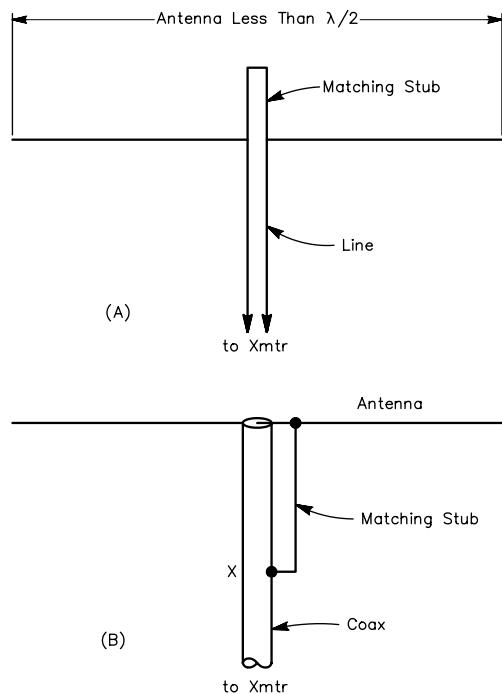
Fig 34—Combined matching stub and balun. The basic arrangement is shown at A. At B, the balun arrangement is achieved by using a section of the outside of the coax feed line as one conductor of a matching stub.
