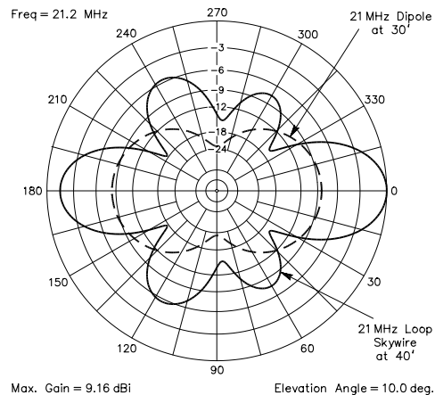
Fig 27—At A, azimuth-plane response of 142-foot long, 7-MHz Loop Skywire, 40 feet in the air at 7.2 MHz, compared with 1/2\text{-}\lambda dipole 30 feet in the air. At B, response of same Loop Skywire at 14.2 MHz, compared with 1/2\text{-}\lambda 14.2-MHz dipole 30 feet in the air. Now the loop has some advantage in certain directions. At C, response of the same Loop Skywire at 21.2 MHz compared to a 21.2-MHz dipole at 30 feet. Here, the Loop Skywire has more gain in almost all directions than the simple dipole. All azimuth-plane patterns were made at 10° elevation.
