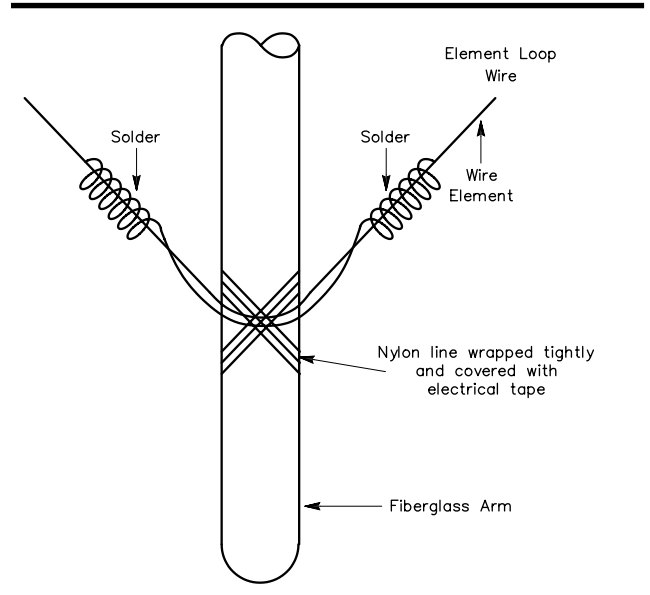
Fig 14—An alternative method of assembling the wire of a quad loop to the spreader arm.
