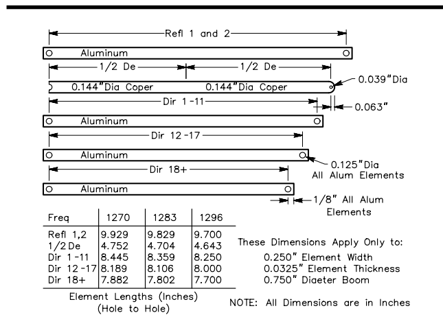
Fig 62—Parasitic elements for the loop Yagi are made from aluminum sheet, the driven element from copper sheet. The dimensions given are for 1/4 -inch wide by 0.0325-inch thick elements only. Lengths specified are hole to hole distances; the holes are located 1/8 inch from each element end.
