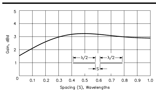
Fig 39—Gain of two collinear \frac{1}{2}\lambda elements as a function of spacing between the adjacent ends.
