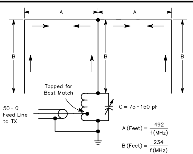
Fig 52 —The bobtail curtain is an excellent low-angle radiator having broadside bidirectional characteristics. Current distribution is represented by the arrows. Dimensions A and B (in feet, for wire antennas) can be determined from the equations.
