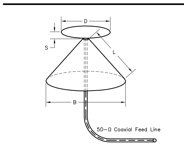
Fig 40—Diagram of VHF/UHF discone, using a sheet-metal disc and cone. It is fed directly with 50- \Omega coax line. The dimensions L and D, together with the spacing S between the disc and cone, determine the frequency characteristics of the antenna. L = 246 / f_{\text{MHz}} for the lowest frequency to be used. Diameter D should be from 0.67 to 0.70 of dimension L. The diameter at the bottom of the cone B is equal to L. The space S between disc and cone can be 2 to 12 inches, with the wider spacing appropriate for larger antennas.
