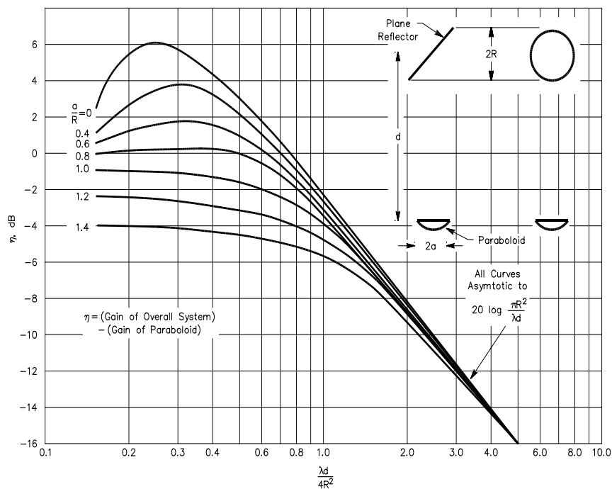
Fig 72—Gain of a periscope antenna using a plane elliptical reflector (after Jasik—see Bibliography).
