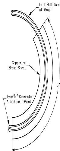
Fig 55—If the match to the antenna cannot be obtained with the tubing alone, a 6-inch piece of copper flashing material can be soldered to the bottom of the first turn of the helix, starting very close to the feed point. The spacing can then be adjusted for best match as described in the text. When the appropriate spacing has been found, affix Teflon or polystyrene blocks between the screen and the winding with silicone sealant to maintain the spacing.
