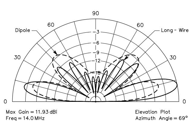
Fig 6—At left, the azimuth responses for a 5-λ long-wire (350 feet long at 14 MHz—solid line) to the same 4-element Yagi (dotted line) and dipole (dashed line) as in Fig 5. Above, the elevation-plane responses for the long-wire (solid line) and the dipole (dashed line) by themselves. Note that the elevation angle giving peak gain for each antenna is just about the same. The long-wire achieves gain by compressing mainly the azimuthal response, squeezing the gain into narrow lobes; not so much by squeezing the elevation pattern for gain.
