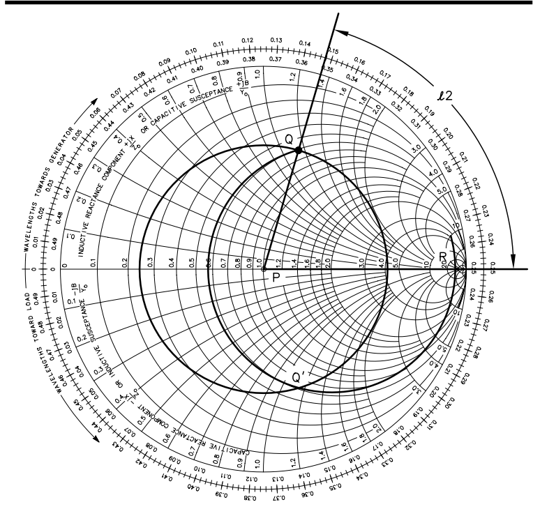
Fig 18—The same impedance locus as shown in Fig 17 except normalized to 75 \Omega instead of 300. The matching circle is now concentric with the chart center, and \ell_2 can be determined directly from the chart, 0.102 \lambda in this case.
