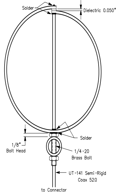
Fig 64—Driven element details. See Fig 62 and the text for additional information.
