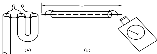
Fig 5—Conversion from unbalanced coax to a balanced load can be done with a \frac{1}{2}\lambda coaxial balun at A. Electrical length of the looped section should be checked with a dip meter, with the ends shorted, as at B. The \frac{1}{2}\lambda balun gives a 4:1 impedance step-up.
