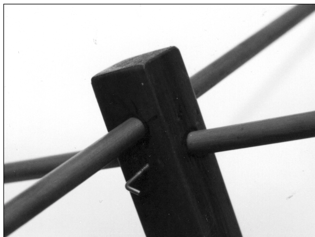
Fig 19—Photo of one end of the VE7CA quad with the two spreaders inserted.
