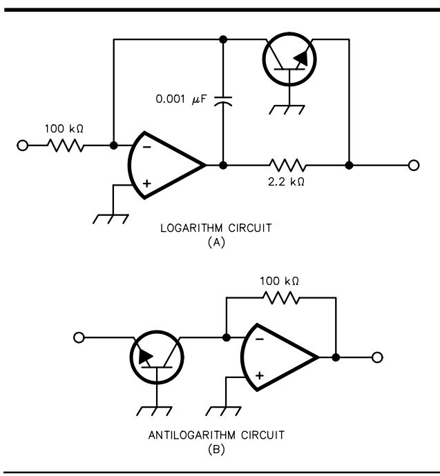
Fig 14 —Simplified diagrams of the log circuit at A and the antilog circuit at B.
