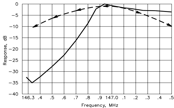
Fig 21—Typical frequency response of a single cavity of the type used in the duplexer. The dotted line represents the passband characteristics of the cavity alone; the solid line for the cavity with a shunt capacitor connected between input and output. An inductance connected in the same manner will cause the rejection notch to be above the frequency to which the cavity is tuned.
