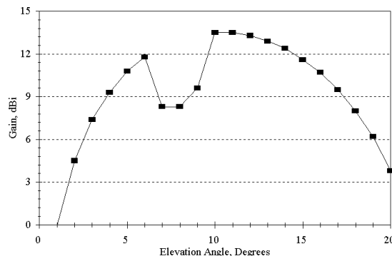
Fig 22 —Elevation response for rays launched at terrain in Fig 21 from a height of 60 feet using a 4-element Yagi. This was computed using a simple Geometrical Optics (GO) reflection-only analysis. Note the “hole” in the response between 6° to 10° in elevation. It is not reasonable for a 10-foot high rock to create such a disturbance at 21 MHz!
