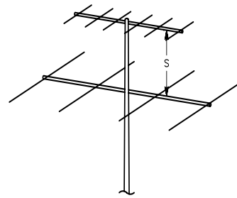
Fig 8—In stacking Yagi arrays one above the other, the minimum spacing between bays (S) should be about half the boom length of the smaller array. Wider spacing is desirable, in which case it should be \frac{1}{2}\lambda , or some multiple thereof, at the frequency of the smaller array. If the beams shown are for 50 and 144 MHz, S should be at least 40 inches, but 80 inches is preferred. Similar conditions apply for stacking antennas for a single band.
