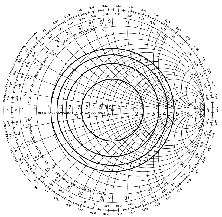
Fig 14—Constant SWR circles for \text{SWR} = 2, 3, 4 and 5 , showing impedance variation along 75\text{-}\Omega line, normalized to 75 \Omega . The actual impedance is obtained by multiplying the chart reading by 75 \Omega .
