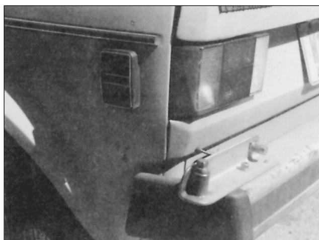
Fig 36—The mount for the mobile J is made from stainless-steel angle stock and secured to the bumper with stainless-steel hardware. Note the 1/2 -inch pipe plug and a PL-259 (with a copper disc soldered in its unthreaded end). These protect the mount and connector threads when the antenna is not in use.
