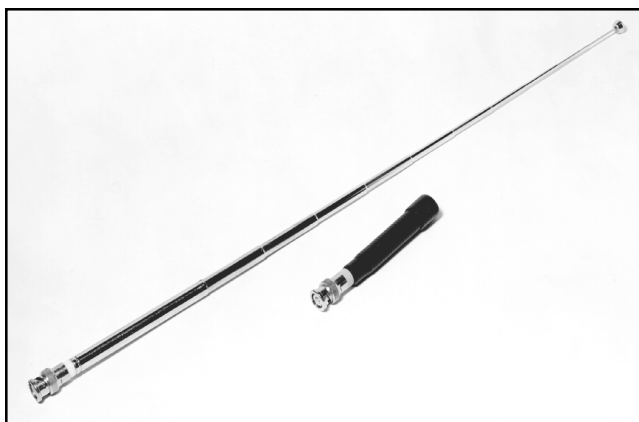
Fig 1 —Two mobile antennas—mobile because they may be used while in motion. Shown here are a telescoping \frac{1}{4}\lambda antenna and a “stubby” antenna, both designed for use at 144 MHz. The \frac{1}{4}\lambda antenna is 19 inch long, while the stubby antenna is only 3\frac{1}{2} inch long. (Both dimensions exclude the length of the BNC connectors. The stubby is a helically wound radiator.
