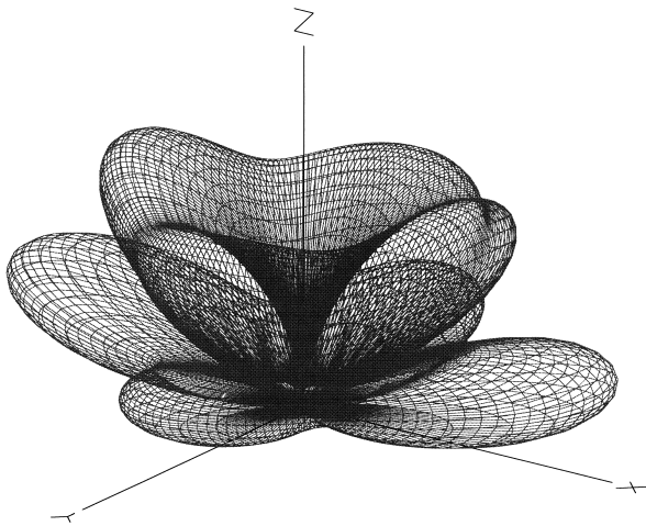
Fig 3—A 3-D representation of the radiation pattern for the 1-λ long-wire shown in Fig 2. The pattern is obviously rather complex. It gets even more complicated for wires longer than 1 λ.
