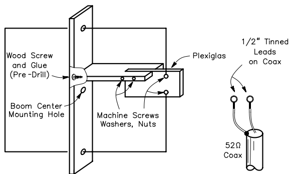
Fig 52—Layout of the driven element of the 144-MHz quad. The leads of the coaxial cable should be stripped to 1/2 inch and solder lugs attached for easy connection and disconnection. See text regarding impedance at loop support points.
