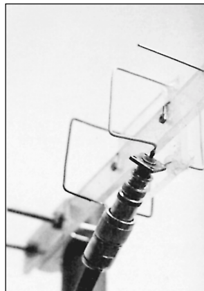
Fig 58—A view of the 10-element version of the 1296-MHz Quagi. It is mounted on a 30-inch Plexiglas boom with a 3 × 3-inch square of Plexiglas to support the driven element and reflector. Note how the driven element is attached to a standard UG-290 BNC connector. The elements are held in place with silicone sealing compound.
