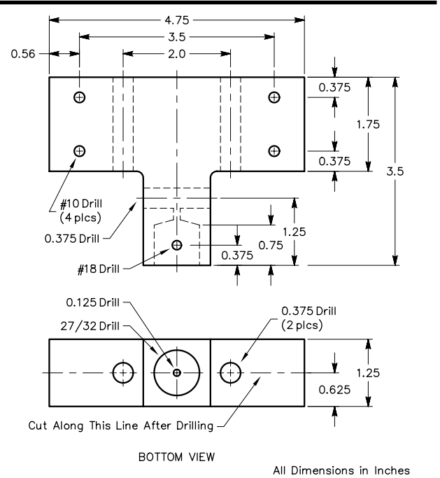
Fig 38—Details of the insulated mounting block. The material is bakelite.
