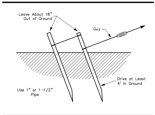
Fig 11—Driven guy anchors. One pipe is usually sufficient for a small mast. For added strength, a second pipe may be added, as shown.
