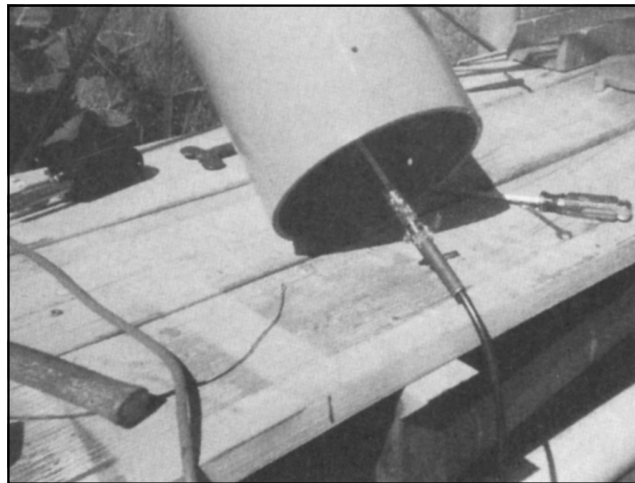
Fig 47—Details of the copper pipe slipped over the feed coax. The coax shield has been folded back over the copper pipe and secured with two stainless-steel hose clamps. The cone wires are also laid against the copper pipe and secured with additional hose clamps.
