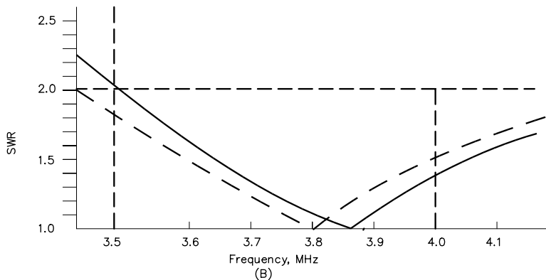
Fig 9— 75/80-meter modified Double Extended Zepp, designed using NEC Wires . At A, a schematic is shown for antenna. At B, SWR curve is shown across 75/80-meter band. Solid line shows measured curve for W7ISV antenna, which was pruned to place SWR minimum higher in the band. The dashed curve shows the computed response when SWR minimum is set to 3.8 MHz.
