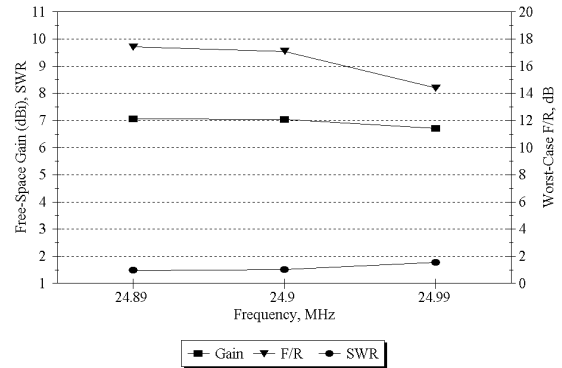
Fig 20 —Computed performance of the pentaband two-element quad on 12 meters.
