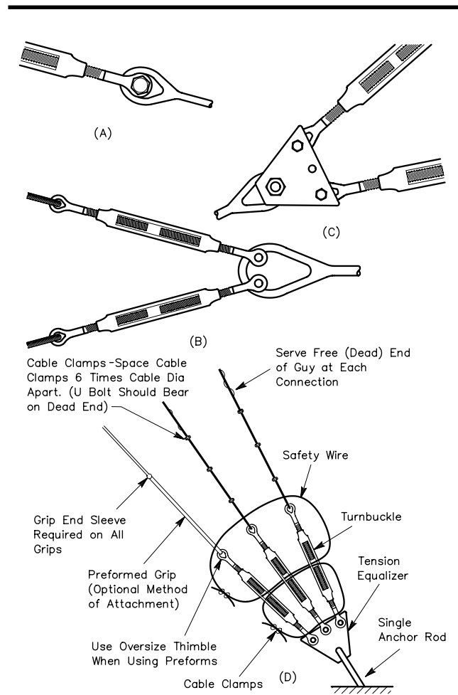
Fig 28—Variety of means available for attaching guy wires and turnbuckles to anchors.
