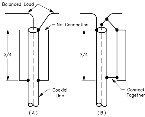
Fig 6—The balun conversion function, with no impedance transformation, can be accomplished with \lambda/4 - \lambda lines, open at the top and connected to the coax outer conductor at the bottom. The coaxial sleeve at A is preferred.
