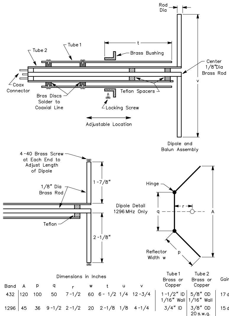
Fig 65—Practical construction information for trough reflector antennas for 432 and 1296 MHz.
