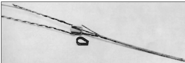
Fig 25—Alternative method for attaching guy wires using dead ends . The dead end on the right is completely assembled (the end of the guy wire extends beyond the grip for illustrative purposes). On the left, one side of the dead end is partially attached to the guy wire. In front, a thimble is used where a sharp bend might cause the guy wire or dead end to break.
