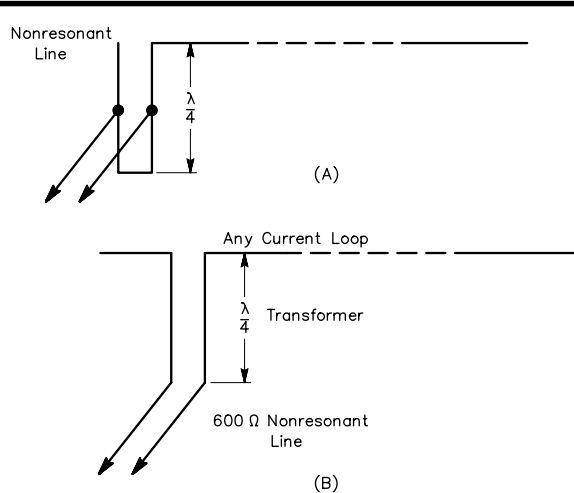
Fig 8—Methods for feeding long single-wire antennas.
