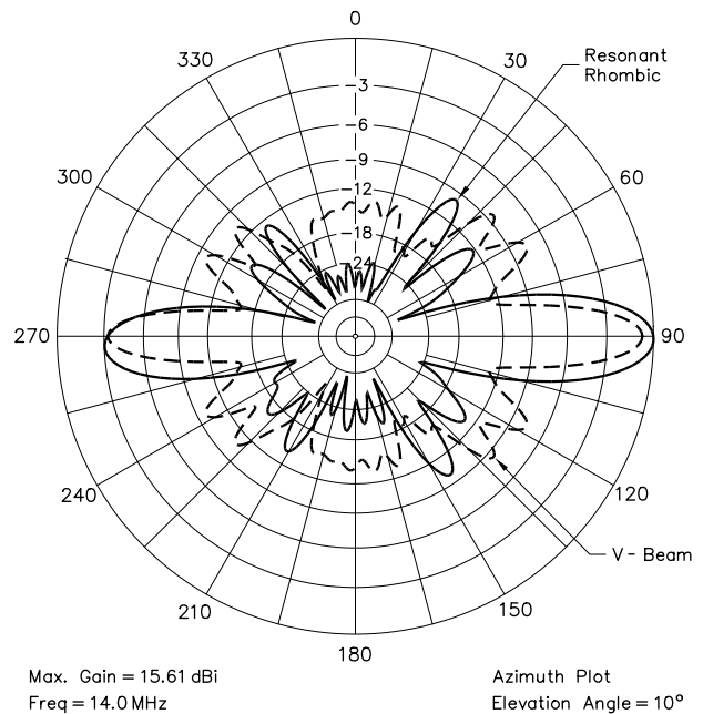
Fig 20—Azimuthal-plane pattern of resonant (underterminated) rhombic (solid line) with 3\lambda legs on 14 MHz, at a height of 70 feet above flat ground, compared with a 6- \lambda per leg V-beam (dashed line) at the same height. Both azimuthal patterns are at a takeoff angle of 10°. The sidelobes for the resonant rhombic are suppressed to a greater degree than those for the V-beam.
