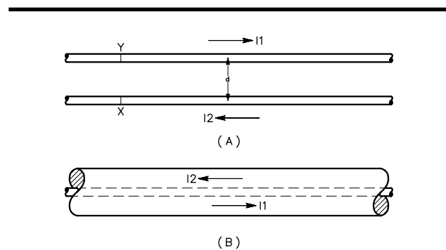
Fig 1—Two basic types of transmission lines.
