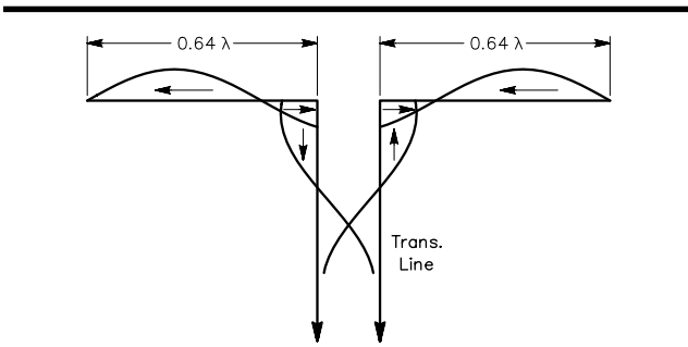
Fig 43 —The extended double Zepp. This system gives somewhat more gain than two \lambda -sized collinear elements.
