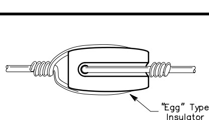
Fig 5—Conventional manner of fastening wire to a strain insulator. This method decreases the leakage path and increases capacitance, as discussed in the text.
