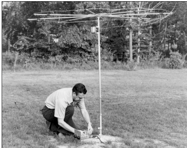
Fig 42—Jerry Sevick, W2FMI, adjusts the 6-foot high, 40-meter vertical.
