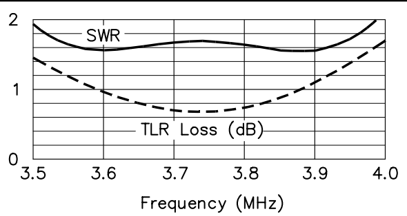
Fig 18 —SWR and loss for a 1 λ 50-Ω feed line. The antenna system model is the one shown in Fig 17.
