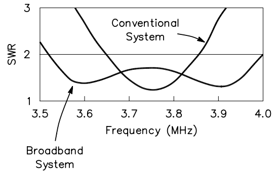
Fig 34—Measured SWR versus frequency for the broadband and conventional antenna systems.
