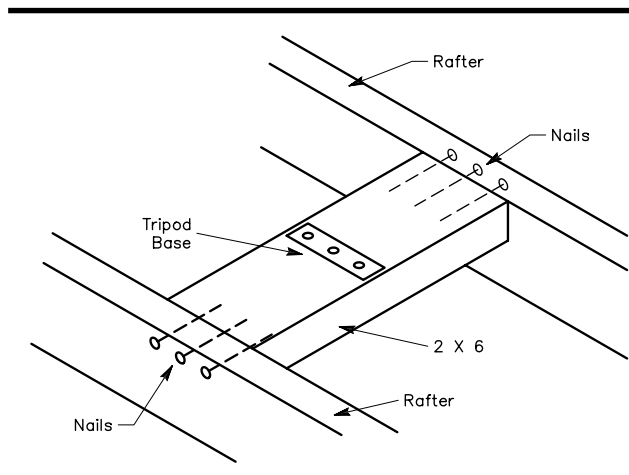
Fig 43 —This cutaway view illustrates how the tripod tower is secured to the roof rafters. The leg to be secured to the crosspiece is placed on the outside of the roof. Another cross member is fastened to the underside of the rafters. Bolts, inserted through the roof and the two cross pieces, hold the inner cross member in place because of pressure applied. The inner crosspiece can be nailed to the rafter for added strength.
