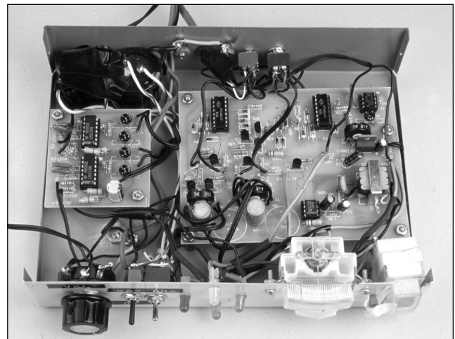
Fig 42—An inside view of one DF unit built into a 2 \times 8 \times 5\frac{3}{4} -inch (HWD) box. Because of the height restriction, the two 4700- \mu F damping capacitors (C8 and C10) are not mounted on the PC board, but near the rear panel behind the smaller of the two PC boards. One of the 4700- \mu F damping capacitors is a standard electrolytic, the other is a parallel combination of five 1000- \mu F, 6.3-V bipolar (nonpolarized) capacitors wrapped in electrical tape.
