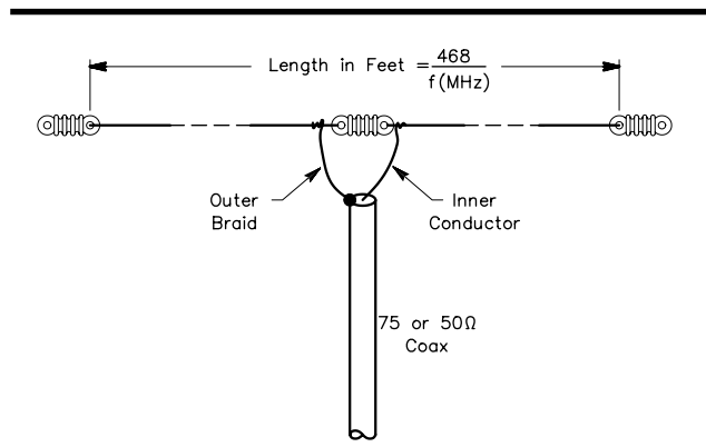
Fig 2—A \lambda/2 - \lambda antenna fed with 75- \Omega coaxial cable. The outside of the outer conductor of the line may be grounded for lightning protection.
