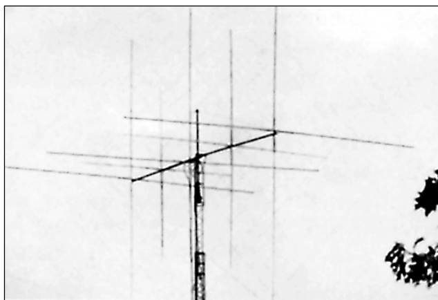
Fig 7 —Photo of the three-band, five-element quad antenna.
