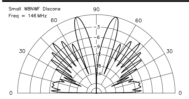
Fig 41—Computed elevation plot over average ground for W8NWF’s small disccone at 146 MHz, ten times its design frequency range. The cone wires are acting as long-wire antennas, distorting severely the low-elevation angle response, even though the feed-point impedance is close to 50 Ω.
