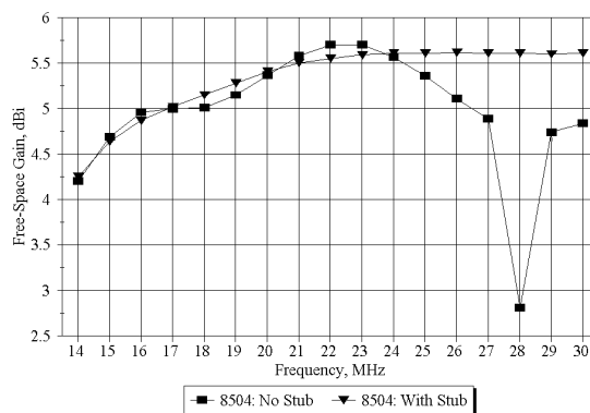
Fig 7—A graph of the gain of model “8504” showing the frequency region in which a “weakness” occurs and its absence once a suitable stub is added to the array.
