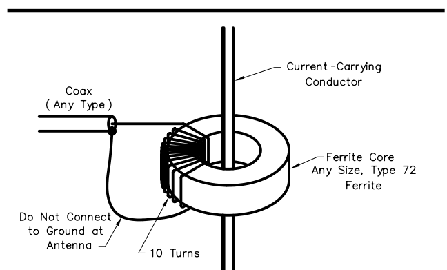
Fig 31 —The current probe for use in the test setup of Fig 30 . The ferrite core is of type 72 material, and may be any size. The coax line must be terminated at the opposite end with a resistor equal to its characteristic impedance.
