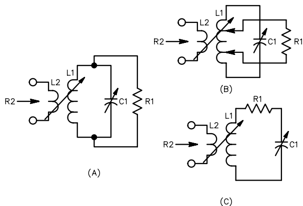
Fig 2—Circuit arrangements for inductively coupled impedance-matching circuit. A and B use a parallel-tuned coupling tank; B is equivalent to A when the taps are at the ends of L1. The series-tuned circuit at C is useful for very low values of load resistance, R1.
