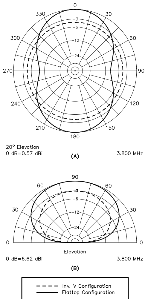
Fig 5—Patterns on 80 meters for 135-foot, center-fed dipole erected as a horizontal flattop dipole at 50 feet, compared with the same dipole installed as an inverted V with the apex at 50 feet and the ends at 10 feet. The azimuth pattern is shown at A, where the dipole wire lies in the 90^\circ to 270^\circ plane. At B, the elevation pattern, the dipole wire comes out of the paper at a right angle. On 80 meters, the patterns are not markedly different from either flattop or inverted-V configuration.
