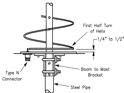
Fig 54—Side view of the helix feed-point assembly. The first half turn of the helix should be kept between 1/4 and 1/2 inch above the ground screen during winding. The height above the screen is adjusted for optimum match to a 52-Ω transmission line after the antenna is completed.
