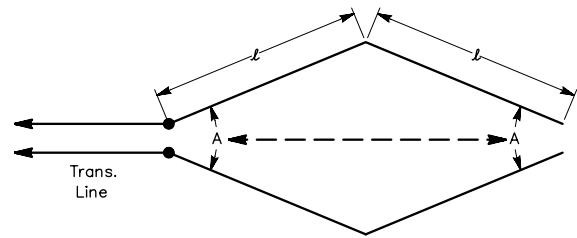
Fig 19—The resonant rhombic or diamond-shaped antenna. All legs are the same length, and opposite angles of the diamond are equal. Length \ell is an integral number of half wavelengths for resonance.
