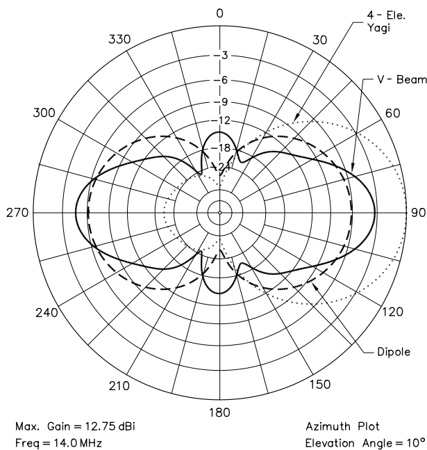
Fig 10—Azimuthal-plane pattern at 10^\circ elevation angle for a 14-MHz V-beam (solid line) with 1\text{-}\lambda legs (68.5 feet long), using an included angle of 75^\circ between the legs. The V-beam is mounted 1 \lambda above flat ground, and is compared with a \frac{1}{2}\text{-}\lambda dipole (dashed line) and a 4-element 20-meter Yagi on a 26-foot boom (dotted line).
