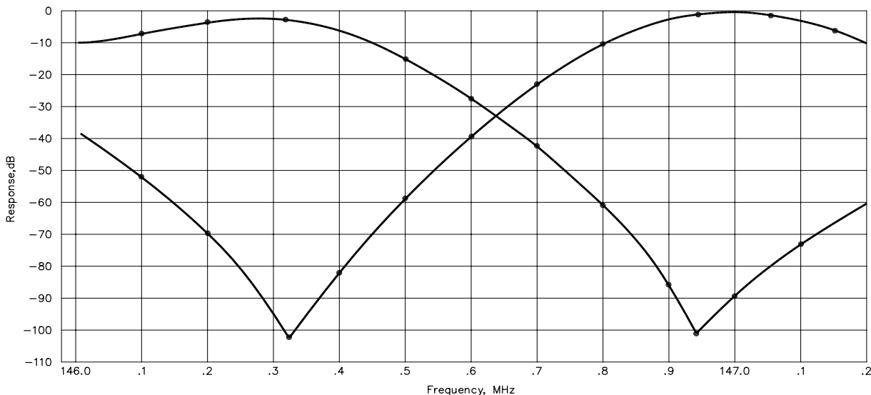
Fig 22—Frequency response of the six-cavity duplexer. One set of three cavities is tuned to pass 146.34 MHz and notch 146.94 MHz (the receiver leg). The remaining set of three cavities is tuned to pass 146.94 MHz and notch 146.34 MHz. This duplexer provides approximately 100 dB of isolation between the transmitter and receiver when properly tuned.
