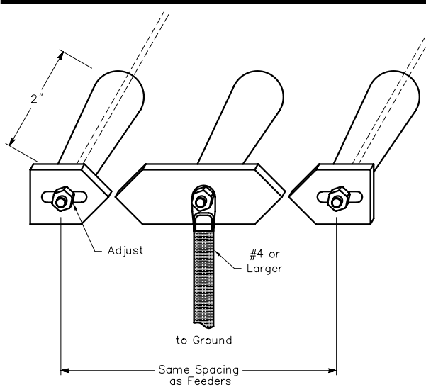
Fig 19—A simple lightning arrester for open-wire line made from three standoff or feedthrough insulators and sections of \frac{1}{8} \times \frac{1}{2} -inch brass or copper strap. It should be installed in the line at the point where the line enters the station. The heavy ground lead should be as short and as direct as possible. The gap setting should be adjusted to the minimum width that will prohibit arcing when the transmitter is operated.
