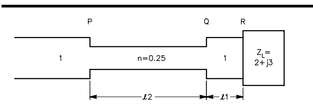
Fig 16—Example for solution by Smith Chart. All impedances are normalized to 300 \Omega .
