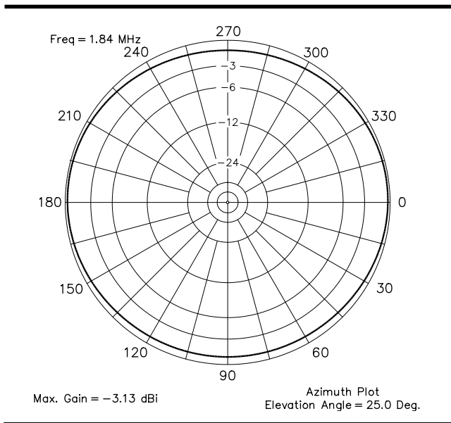
Fig 54—Azimuthal pattern for the inverted L with a single radial at an elevation angle of 25°.
