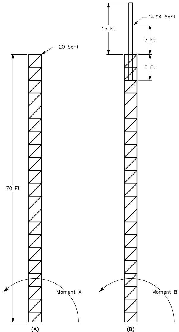
Fig 31 —At A, a 70-foot tower rated for 20 square feet of antenna load at the top. At B, the same tower with a 2-inch OD x 20-foot long mast, with an antenna mounted 7 feet above the top of the tower. Both configurations produce the same tower load.
