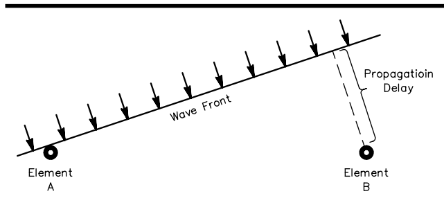
Fig 11—This diagram illustrates one technique used in electronic beam forming. By delaying the signal from element A by an amount equal to the propagation delay, the two signals may be summed precisely in phase, even though the signal is not in the broadside direction. Because this time delay is identical for all frequencies, the system is not frequency sensitive.
