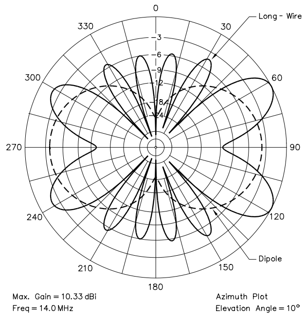
Fig 4—An azimuthal-plane comparison between a 3-λ (209 feet long) long-wire (solid line) and the comparison 1/2-λ dipole (dashed line) at 70 feet high (1 λ) at 14 MHz.
