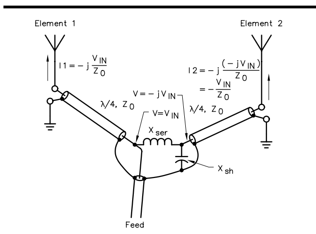
Fig 18—Quadrature feed system. Equations in the text permit calculation of values for the L network components, X_{\text{ser}} and X_{\text{sh}} .
