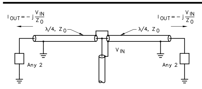
Fig 17—A useful property of \lambda/4 -λ transmission lines; see text. This property is utilized in the “current forcing” method of feeding an array of coupled elements.
