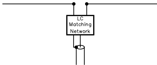
Fig 20 —Efficient broadband matching with an lumped element LC network. The antenna in this example has a resistance of 72 \Omega and a Q of 12. The matching network has an impedance level of 12.4 \Omega , and a Q of 200. The feed line is 50- \Omega coax, and the matching network provides an impedance step-up ratio of 2.8:1.
