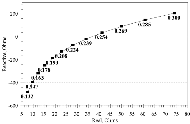
Fig 24—Feed-point impedance for the same antennas as in Fig 21, but calibrated in wavelength rather than frequency, over the range from 0.132λ to 0.300λ, above and below the quarter-wave resonance.
