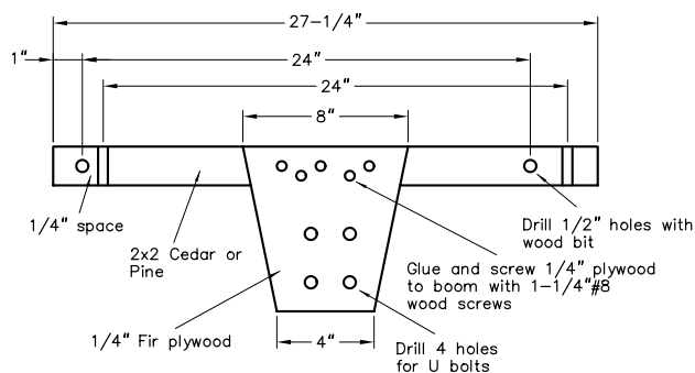
Fig 18—Dimensions for boom and the boom-to-mast bracket for VE7CA's portable two-element 6-meter quad.
