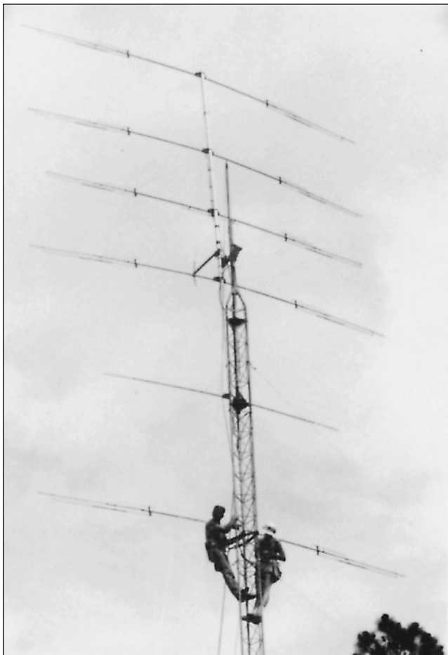
Fig 40—Mounting the last element prior to positioning the boom in a horizontal plane.
