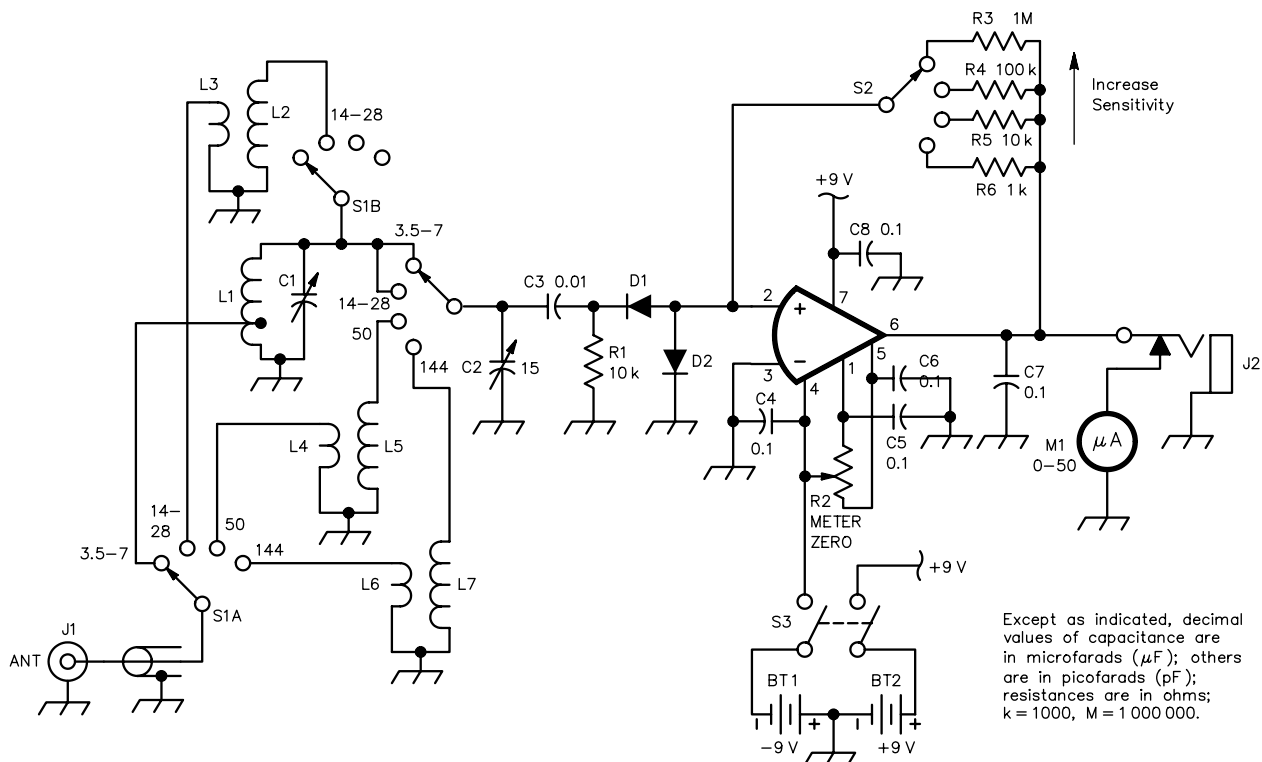
Fig 56—Circuit diagram of the linear field strength meter. All resistors are 1/4- or 1/2-W composition types.
