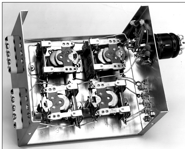
Fig 62 —Inside view of relay box. Four relays provide control over five antennas. See text. The relays pictured here are Potter and Brumfeld type MR11D.
