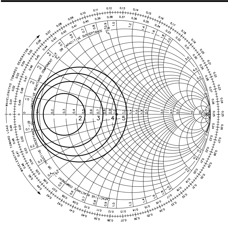
Fig 15—Paths of constant SWR for SWR = 2, 3, 4 and 5, showing impedance variation along 75- \Omega line, normalized to 300 \Omega . Normalized impedances differ from those in Fig 14, but actual impedances are obtained by multiplying chart readings by 300 \Omega and are the same as those corresponding in Fig 14. Paths remain circles but are no longer concentric. One, the matching circle, SWR = 4 in this case, passes through the chart center and is thus the locus of all impedances which can be matched to a 300- \Omega line.
