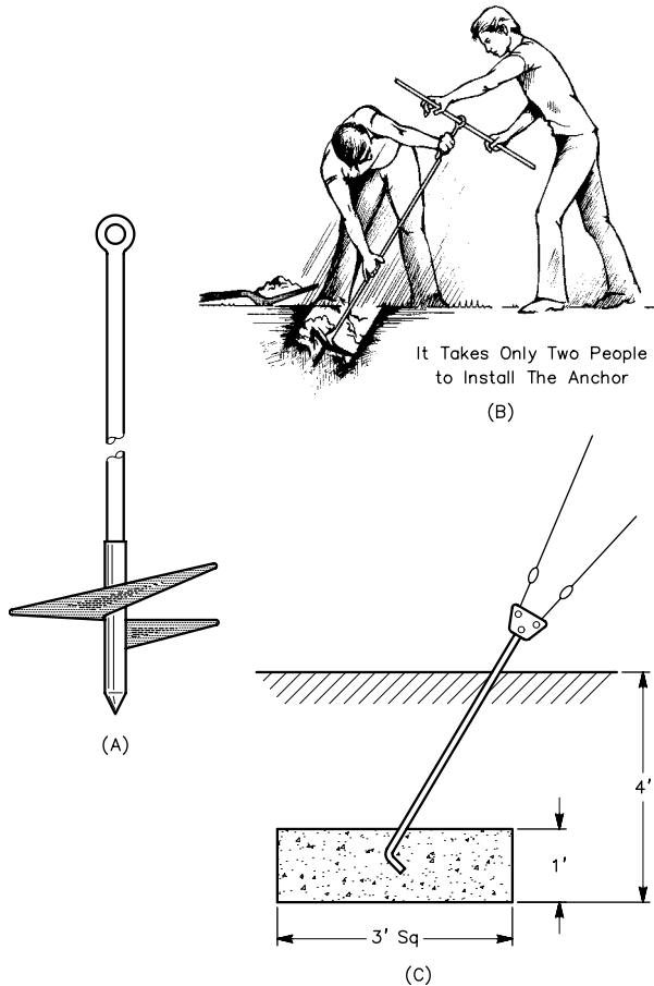
Fig 27—Two standard types of guy anchors. The earth screw shown at A is easy to install and widely available, but may not be suitable for use in certain soils. The concrete anchor is more difficult to install properly, but it is suitable for use with a wide variety of soil conditions and will satisfy most building code requirements.
